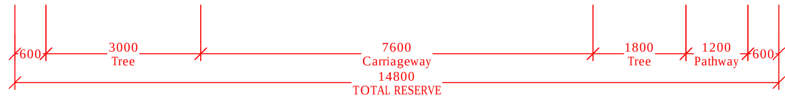
INDICATIVE 14.8m LOCAL MINOR ROAD STREETSCAPE (ROADS 402,403, 404, 405, 407, 408) SCALE 1:75
