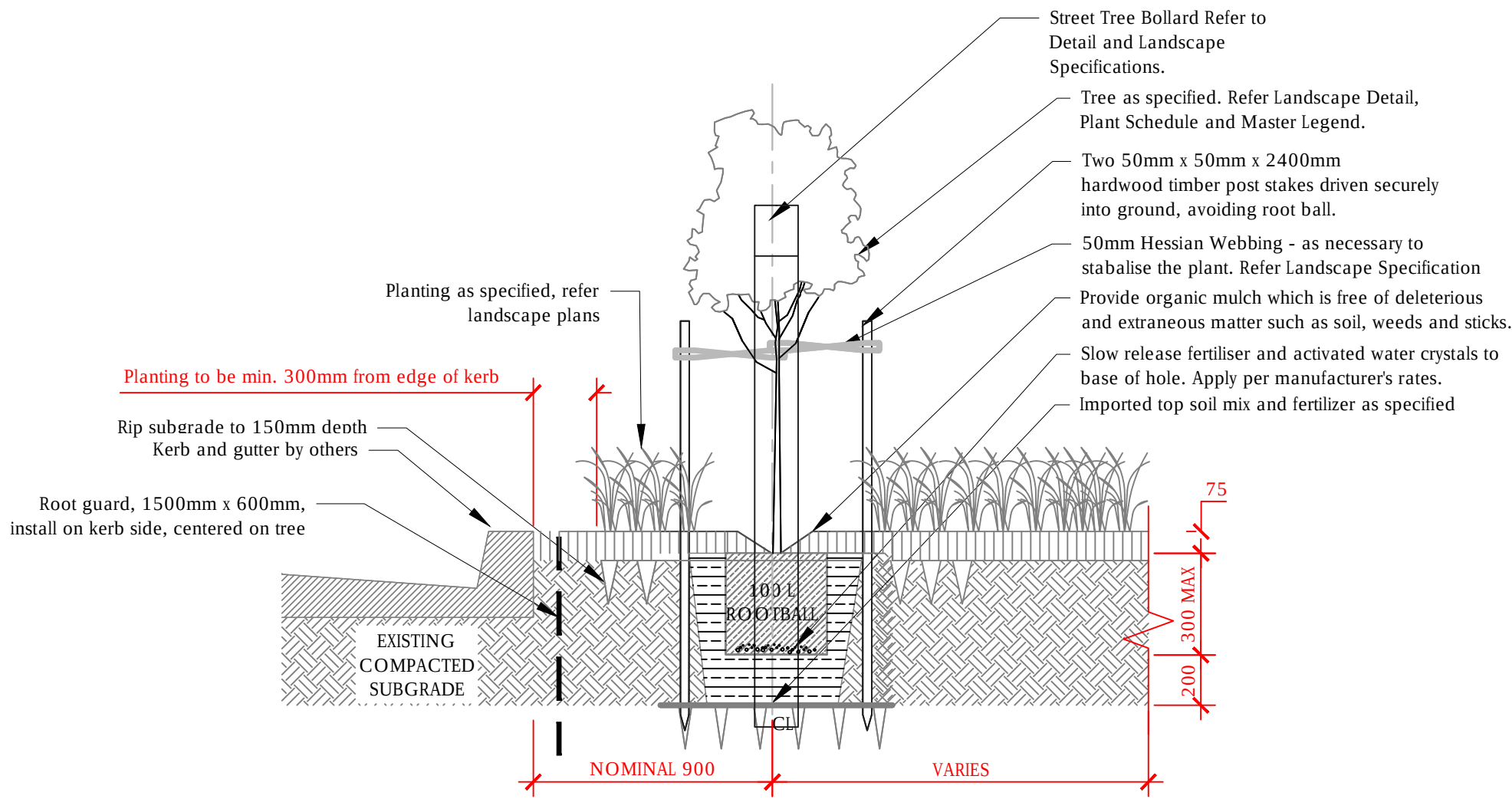
TYPICAL STREET TREE IN BLISTER DETAIL - LOCAL ROAD SCALE 1:20
